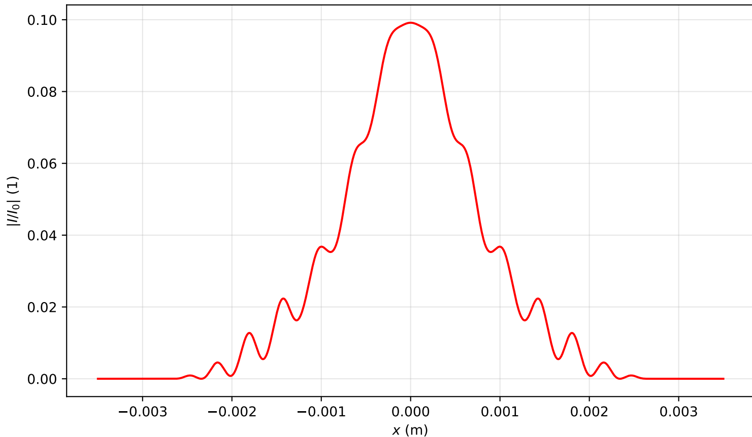
Intensity profile I(x, y = 0, z = 2.548)/I_0 , P_{in}=2.0P_{cr} , artificial time
